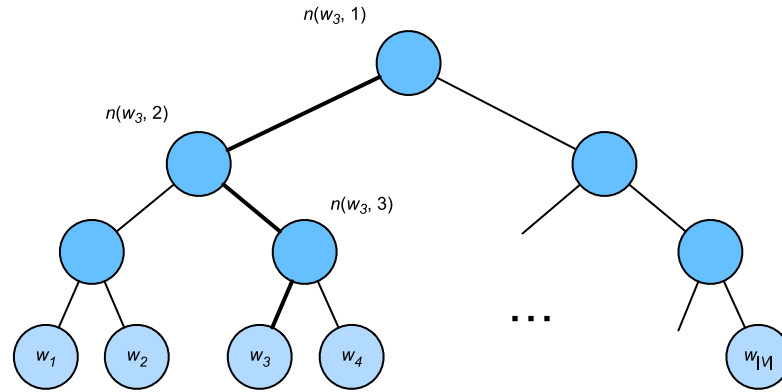
Figure 15.2.1 Hierarchical softmax for approximate training, where each leaf node of the tree represents a word in the dictionary.
