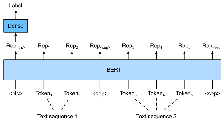
Figure 16.6.2 Fine-tuning BERT for text pair classification or regression applications, such as natural language inference and semantic textual similarity. Suppose that the input text pair has two and three tokens.
