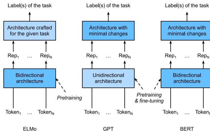
Figure 15.8.1 A comparison of ELMo, GPT, and BERT.
