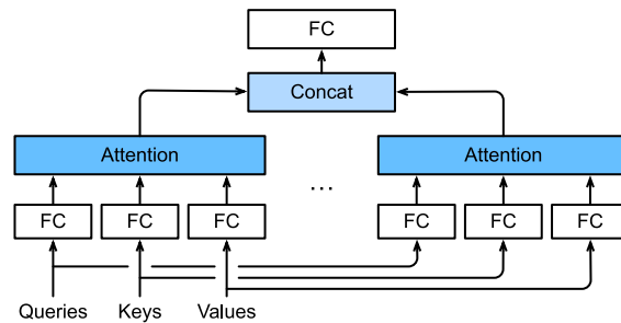
Figure 11.5.1 Multi-head attention, where multiple heads are concatenated then linearly transformed.
