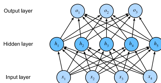
Figure 5.1.1 An MLP with a hidden layer of 5 hidden units.
