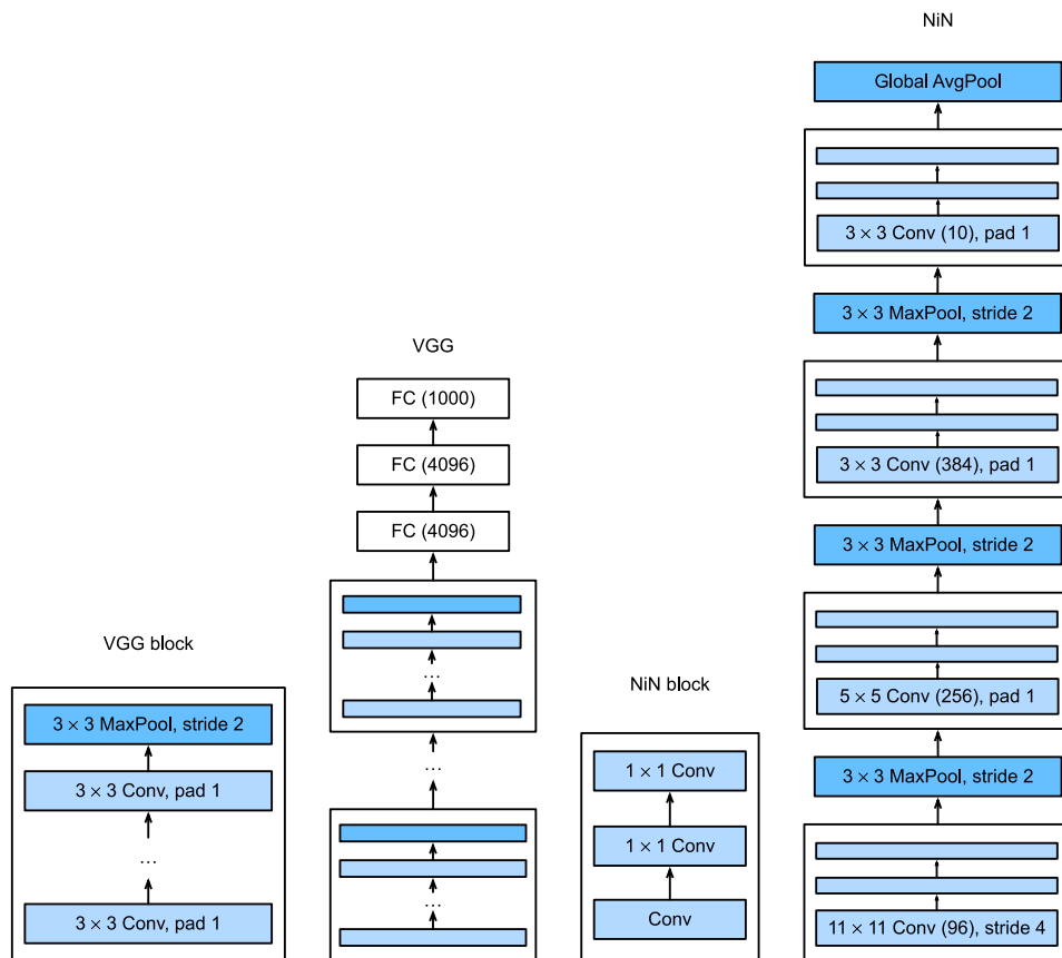
Figure 8.3.1 Comparing the architectures of VGG and NiN, and of their blocks.
