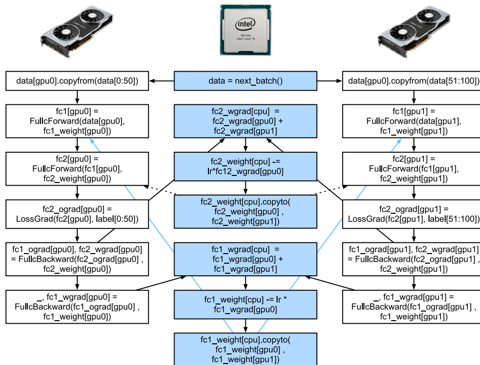
Figure 13.3.1 The computational graph and its dependencies of a two-layer MLP on a CPU and two GPUs.
