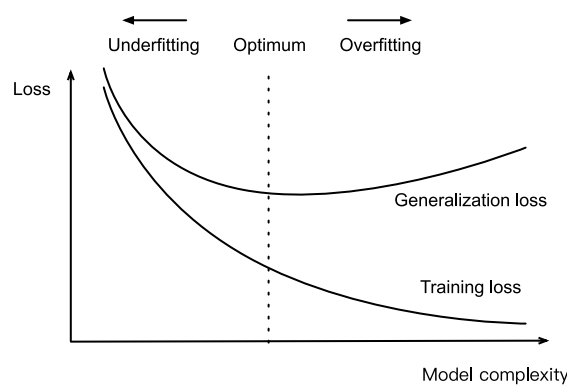
Figure 3.6.1 Influence of model complexity on underfitting and overfitting
