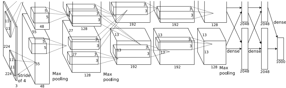
Figure 13.5.1 Model parallelism in the original AlexNet design due to limited GPU memory.
