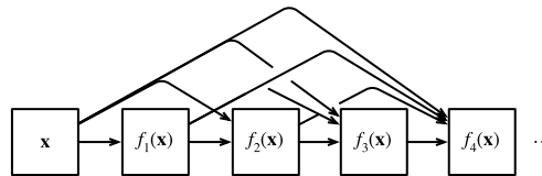
Figure 8.7.2 Dense connections in DenseNet. Note how the dimensionality increases with depth.
