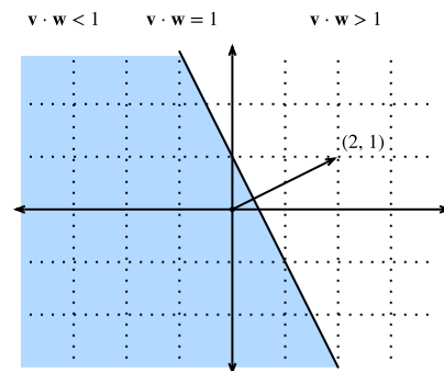
Figure 19.1.6 If we now consider the inequality version of the expression, we see that our hyperplane (in this case: just a line) separates the space into two halves.
