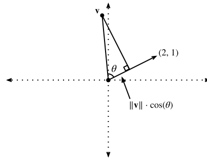
Figure 19.1.5 Recalling trigonometry, we see the formula \|v\| \cos(\theta) is the length of the projection of the vector v onto the direction of w
