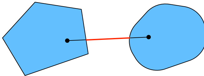
Figure 12.2.3 The union of two convex sets need not be convex.
