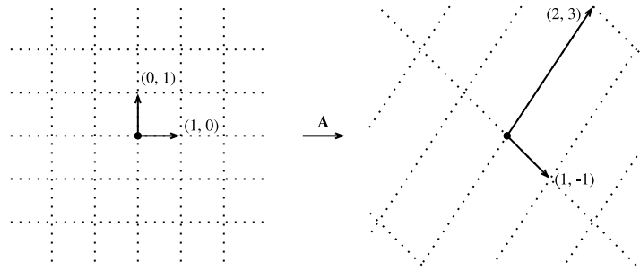
Figure 19.1.8 The matrix A acting on the given basis vectors. Notice how the entire grid is transported along with it.
