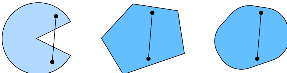
Figure 12.2.1 The first set is nonconvex and the other two are convex.
