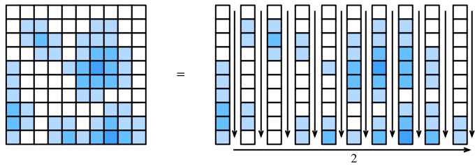
Figure 19.5.3 Illustrating how to decompose a sum over many squares as a sum over first the columns (1), then adding the column sums together (2).
