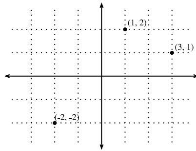
Figure 19.1.1 An illustration of visualizing vectors as points in the plane. The first component of the vector gives the x-coordinate, the second component gives the y-coordinate. Higher dimensions are analogous, although much harder to visualize.
