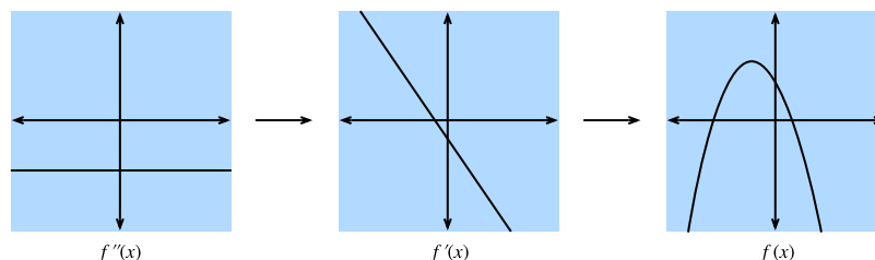
Figure 19.3.2 If we assume the second derivative is a negative constant, then the first derivative is decreasing, which implies the function itself has a maximum.
