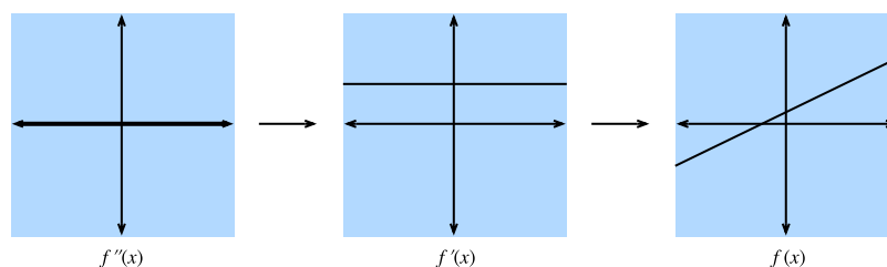
Figure 19.3.3 If we assume the second derivative is zero, then the first derivative is constant, which implies the function itself is a straight line.
