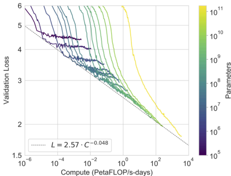
Figure 11.8.1 GPT-3 performance (cross-entropy validation loss) follows a power-law trend with the amount of compute used for training. The power-law behavior observed in Kaplan et al. (2020) continues for an additional two orders of magnitude with only small deviations from the predicted curve. Embedding parameters are excluded from compute and parameter counts (caption adapted and figure taken from Brown et al. (2020)).
