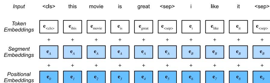
Figure 15.8.2 The embeddings of the BERT input sequence are the sum of the token embeddings, segment embeddings, and positional embeddings.
