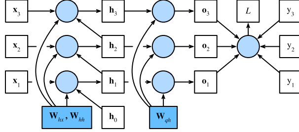
Figure 9.7.2 Computational graph showing dependencies for an RNN model with three time steps. Boxes represent variables (not shaded) or parameters (shaded) and circles represent operators.
