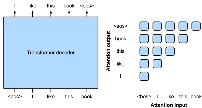
Figure 11.8.6 Left: Pretraining GPT with language modeling. The target sequence is the input sequence shifted by one token. Both <bos> and <eos> are special tokens marking the beginning and end of sequences, respectively. Right: Attention pattern in the transformer decoder. Each token along the vertical axis attends to only its past tokens along the horizontal axis (causal).
