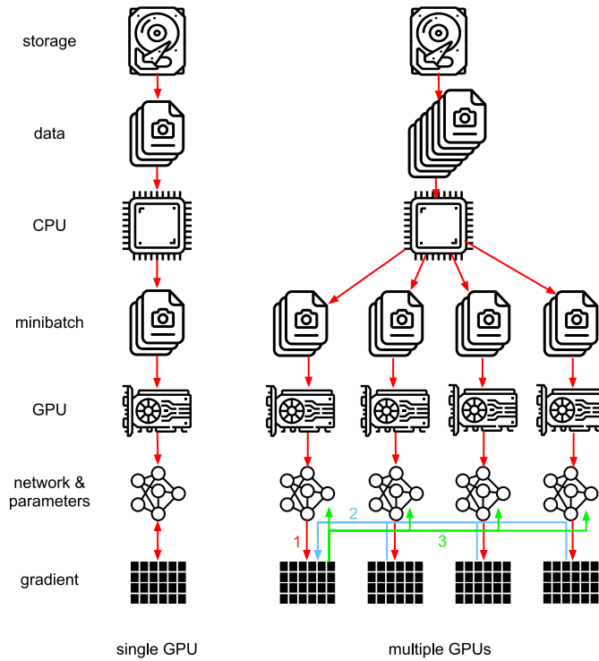
Figure 13.7.1 Left: single GPU training. Right: a variant of multi-GPU training: (1) we compute loss and gradient, (2) all gradients are aggregated on one GPU, (3) parameter update happens and the parameters are re-distributed to all GPUs.
