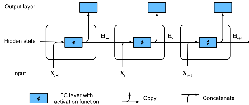
Figure 9.4.1 An RNN with a hidden state.
