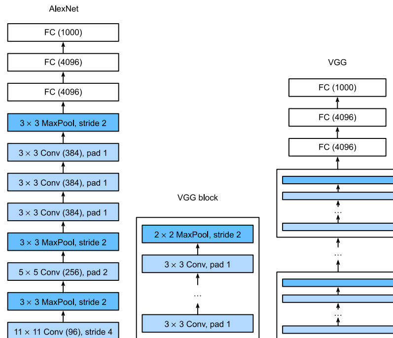
Figure 8.2.1 From AlexNet to VGG. The key difference is that VGG consists of blocks of layers, whereas AlexNets layers are all designed individually.
