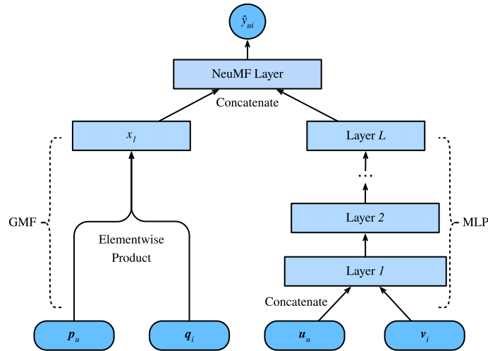
Figure 17.6.1 Illustration of the NeuMF model
