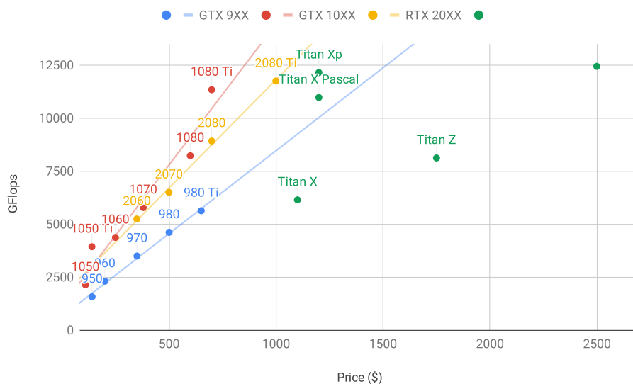
Figure 20.5.1 Floating-point compute power and price comparison.
