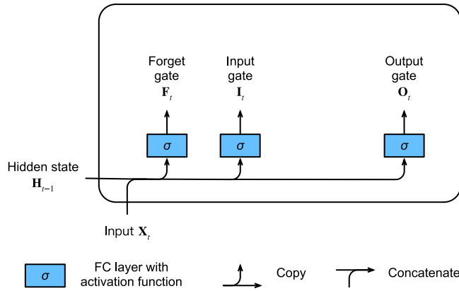
Figure 10.1.1 Computing the input gate, the forget gate, and the output gate in an LSTM model.
