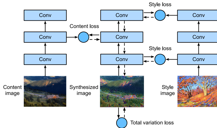
Figure 14.12.2 CNN-based style transfer process. Solid lines show the direction of forward propagation and dotted lines show backward propagation.
