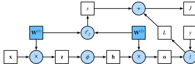
Figure 5.3.1 Computational graph of forward propagation.
