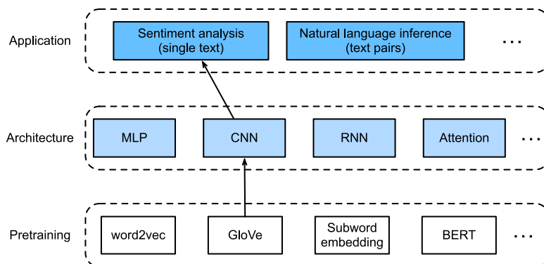
Figure 16.3.1 This section feeds pretrained GloVe to a CNN-based architecture for sentiment analysis.
