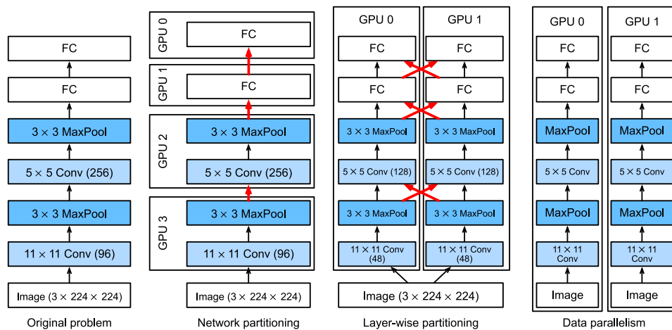
Figure 13.5.2 Parallelization on multiple GPUs. From left to right: original problem, network partitioning, layerwise partitioning, data parallelism.
