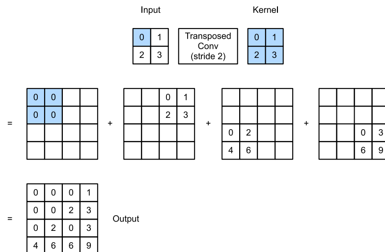
Figure 14.10.2 Transposed convolution with a 2 \times 2 kernel with stride of 2. The shaded portions are a portion of an intermediate tensor as well as the input and kernel tensor elements used for the computation.
