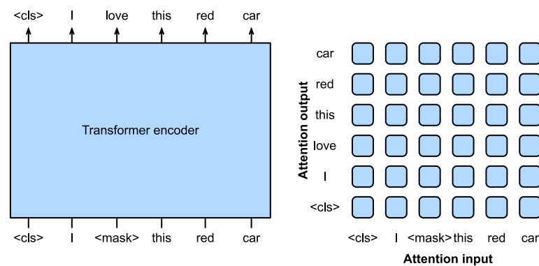
Figure 11.8.1 Left: Pretraining BERT with masked language modeling. Prediction of the masked love token depends on all input tokens before and after love. Right: Attention pattern in the transformer encoder. Each token along the vertical axis attends to all input tokens along the horizontal axis.
