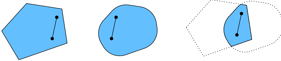
Figure 12.2.2 The intersection between two convex sets is convex.
