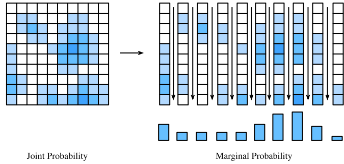
Figure 19.6.1 By summing along the columns of our array of probabilities, we are able to obtain the marginal distribution for just the random variable represented along the x-axis.
