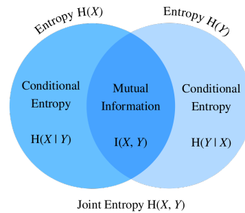
Figure 19.11. Mutual informations relationship with joint entropy and conditional entropy.
