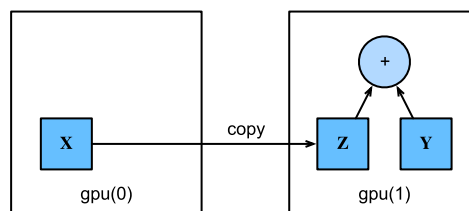
Figure 6.7.1 Copy data to perform an operation on the same device.
