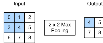
Figure 7.5.1 Max-pooling with a pooling window shape of 2 \times 2 . The shaded portions are the first output element as well as the input tensor elements used for the output computation: \max(0, 1, 3, 4) = 4 .
