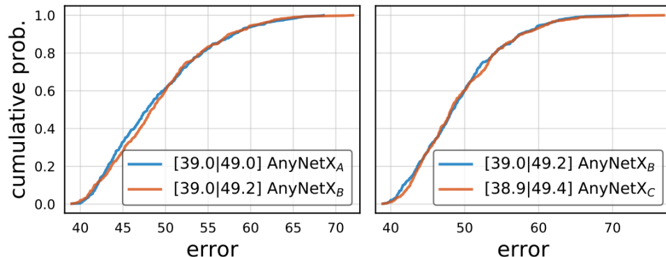
Figure 8.8.2 Comparing error empirical distribution functions of design spaces. The legends show the min error and mean error. Sharing bottleneck ratio (from AnyNetX A to AnyNetX B ) and sharing the number of groups (from AnyNetX B to AnyNetX C ) simplify the design space with virtually no change in error distributions (figure taken from Radosavovic et al. (2020)).
