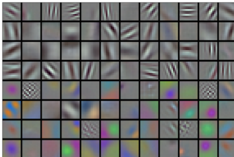
Figure 8.1.1 Image filters learned by the first layer of AlexNet. Reproduction courtesy of Krizhevsky et al. (2012).
