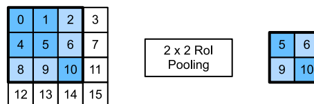
Figure 14.8.3 A 2 \times 2 region of interest pooling layer.
