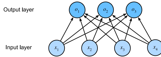
Figure 4.1.1 Softmax regression is a single-layer neural network.
