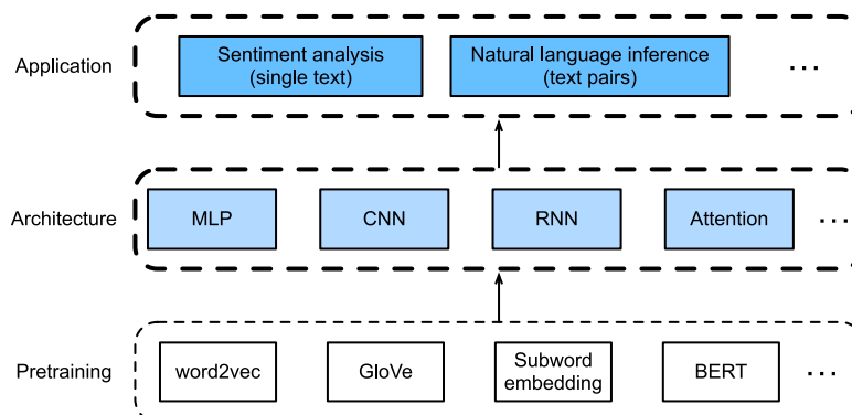
Figure 16.1 Pretrained text representations can be fed to various deep learning architectures for different downstream natural language processing applications. This chapter focuses on how to design models for different downstream natural language processing applications.
