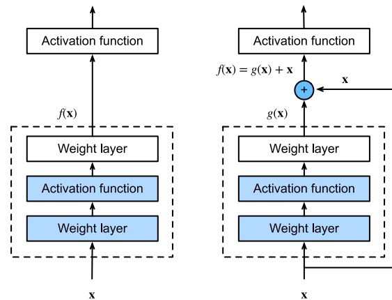
Figure 8.6.2 In a regular block (left), the portion within the dotted-line box must directly learn the mapping f(x) . In a residual block (right), the portion within the dotted-line box needs to learn the residual mapping g(x) = f(x) - x , making the identity mapping f(x) = x easier to learn.
