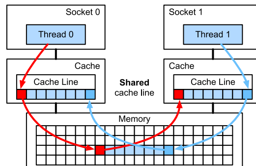
Figure 13.4.6 False sharing (image courtesy of Intel).
