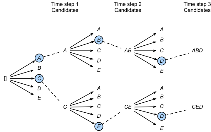
Figure 10.8.3 The process of beam search (beam size: 2, maximum length of an output sequence: 3). The candidate output sequences are A, C, AB, CE, ABD, and CED.
