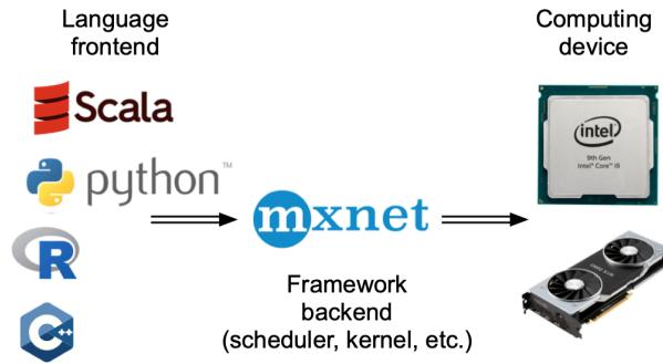
Figure 13.2.1 Programming language frontends and deep learning framework backends.
