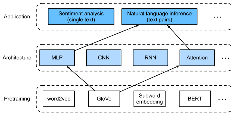
Figure 16.5.1 This section feeds pretrained GloVe to an architecture based on attention and MLPs for natural language inference.
