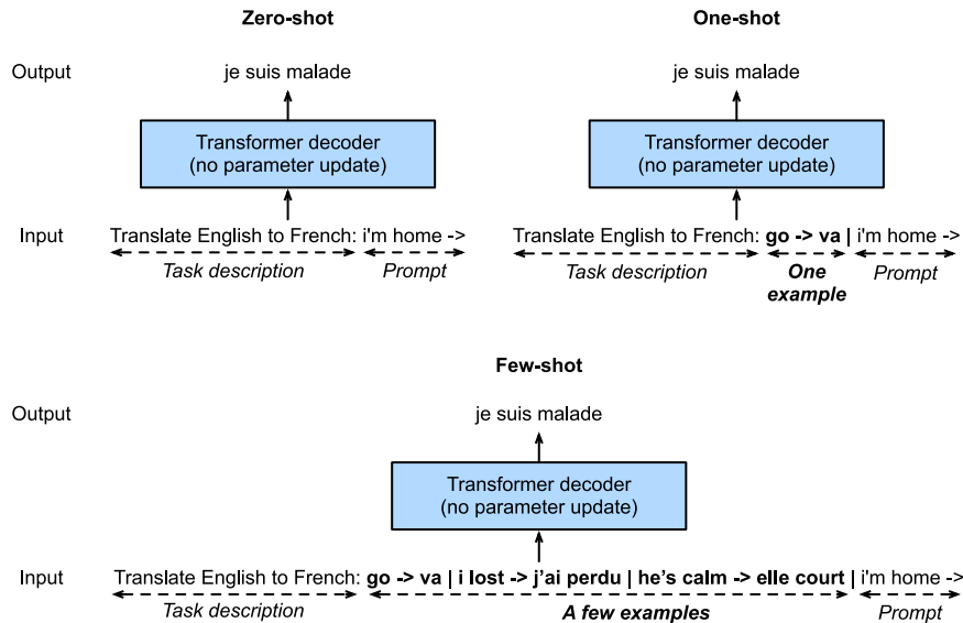
Figure 11.8.7 Zero-shot, one-shot, few-shot learning with language models (transformer decoders). No parameter update is needed.
