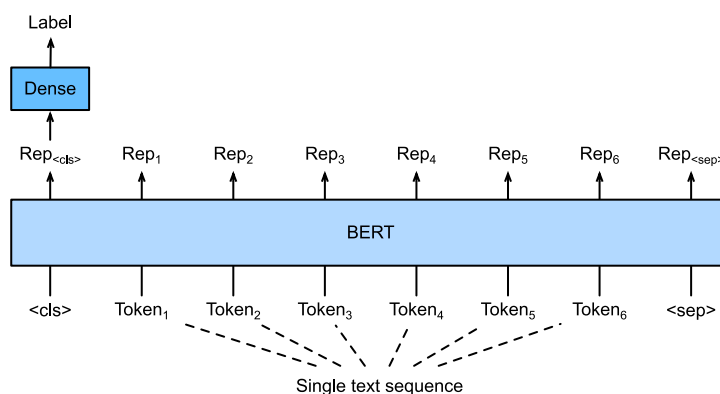
Figure 16.6.1 Fine-tuning BERT for single text classification applications, such as sentiment analysis and testing linguistic acceptability. Suppose that the input single text has six tokens.
