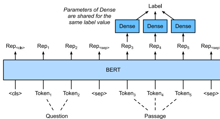
Figure 16.6.4 Fine-tuning BERT for question answering. Suppose that the input text pair has two and three tokens.
