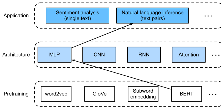
Figure 16.7.1 This section feeds pretrained BERT to an MLP-based architecture for natural language inference.
