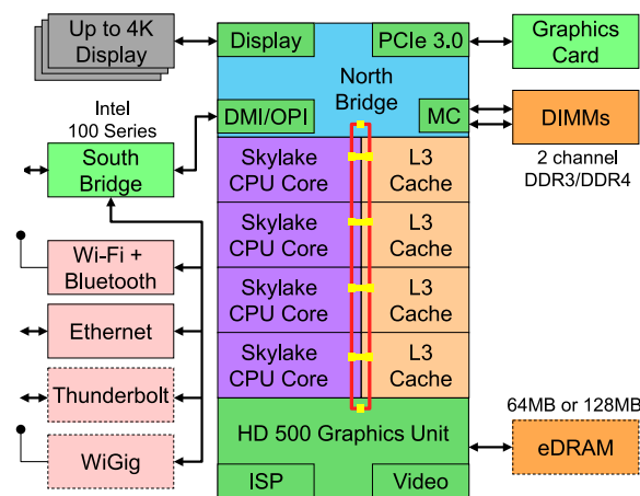
Figure 13.4.3 Intel Skylake consumer quad-core CPU.
