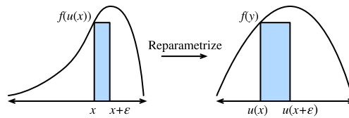
Figure 19.5.2 Visualizing the transformation of a single thin rectangle under the change of variables.
