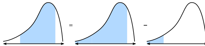
Figure 19.5.1 Visualizing why we may reduce the problem of computing the area under a curve between two points to computing the area to the left of a point.
