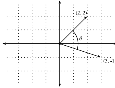
Figure 19.1.4 Between any two vectors in the plane there is a well defined angle \theta . We will see this angle is intimately tied to the dot product.
