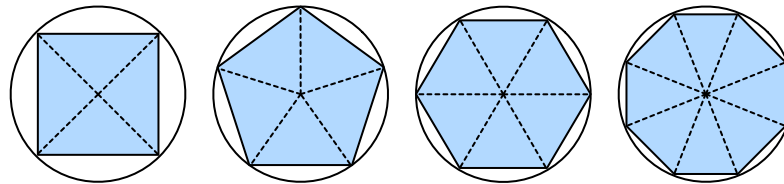
Figure 2.4.1 Finding the area of a circle as a limit procedure.
