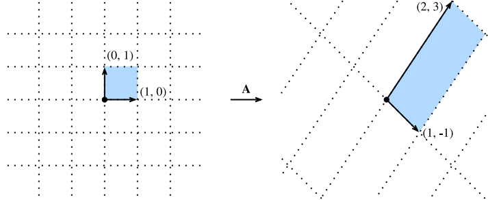
Figure 19.1.9 The matrix A again distorting the grid. This time, I want to draw particular attention to what happens to the highlighted square.
