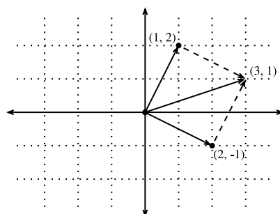
Figure 19.1.3 We can visualize vector addition by first following one vector, and then another.
