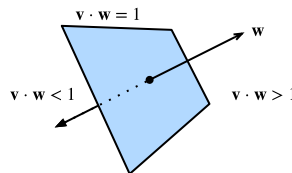
Figure 19.1.7 Hyperplanes in any dimension separate the space into two halves.
