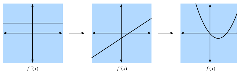
Figure 19.3.1 If we assume the second derivative is a positive constant, then the first derivative is increasing, which implies the function itself has a minimum.
