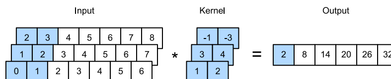
Figure 16.3.3 One-dimensional cross-correlation operation with 3 input channels. The shaded portions are the first output element as well as the input and kernel tensor elements used for the output computation: 0 \times 1 + 1 \times 2 + 1 \times 3 + 2 \times 4 + 2 \times (-1) + 3 \times (-3) = 2 .
