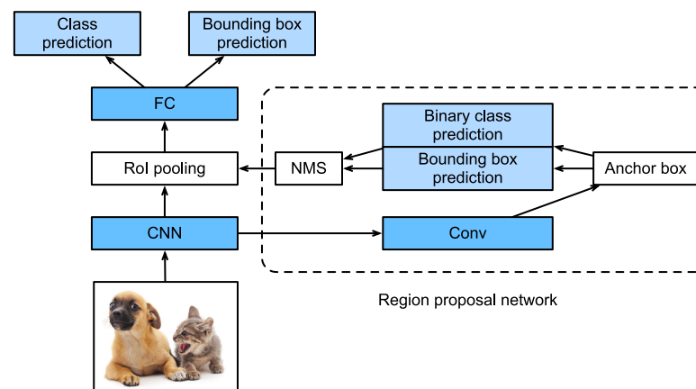
Figure 14.8.4 The faster R-CNN model.
