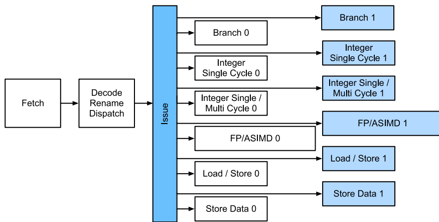
Figure 13.4.4 ARM Cortex A77 Microarchitecture.
