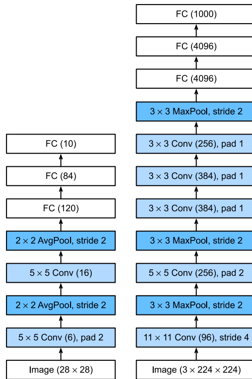
Figure 8.1.2 From LeNet (left) to AlexNet (right).
