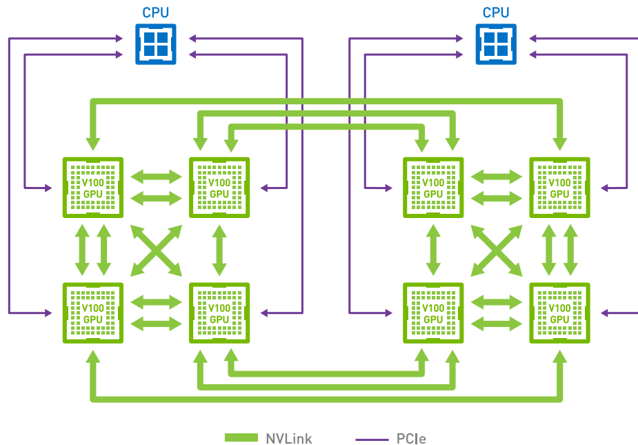
Figure 13.7.4 NVLink connectivity on 8 V100 GPU servers (image courtesy of NVIDIA).
