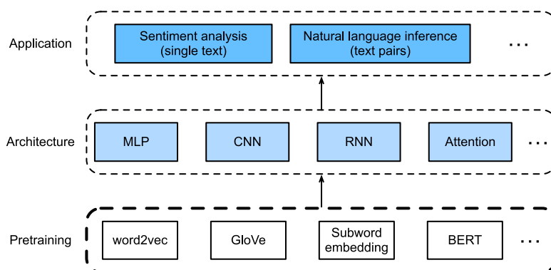
Figure 15.1 Pretrained text representations can be fed to various deep learning architectures for different downstream natural language processing applications. This chapter focuses on the upstream text representation pretraining.
