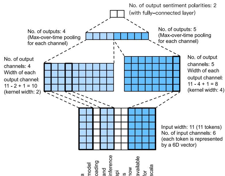
Figure 16.3.5 The model architecture of textCNN.
