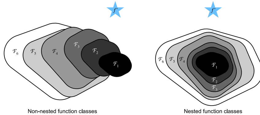
Figure 8.6.1 For non-nested function classes, a larger (indicated by area) function class does not guarantee to get closer to the truth function ( f^* ). This does not happen in nested function classes.
