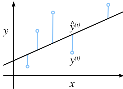
Figure 3.1.1 Fitting a linear regression model to one-dimensional data.
