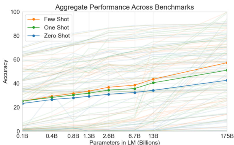
Figure 11.8.8 Aggregate performance of GPT-3 for all 42 accuracy-denominated benchmarks (caption adapted and figure taken from Brown et al. (2020)).
