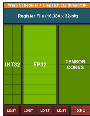
Figure 13.4.7 NVIDIA Turing processing block (image courtesy of NVIDIA).
