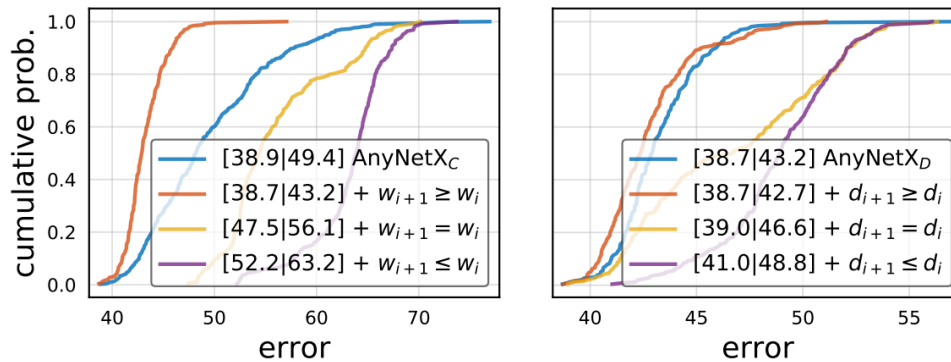
Figure 8.8.3 Comparing error empirical distribution functions of design spaces. The legends show the min error and mean error. Increasing network width across stages (from AnyNetX C to AnyNetX D ) and increasing network depth across stages (from AnyNetX D to AnyNetX E ) simplify the design space with improved error distributions (figure taken from Radosavovic et al. (2020)).
