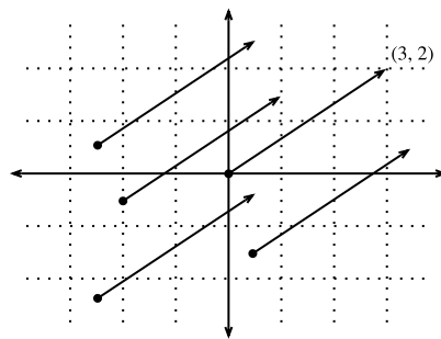
Figure 19.1.2 Any vector can be visualized as an arrow in the plane. In this case, every vector drawn is a representation of the vector (3, 2)^\top .
