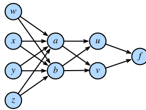
Figure 19.4.1 The function relations above where nodes represent values and edges show functional dependence.
