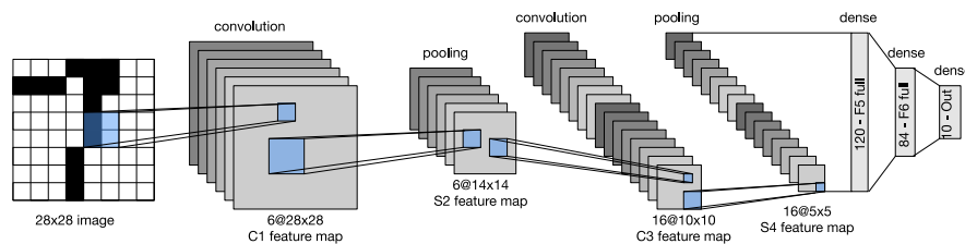
Figure 7.6.1 Data flow in LeNet. The input is a handwritten digit, the output a probability over 10 possible outcomes.
