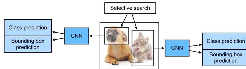
Figure 14.8.1 The R-CNN model.
