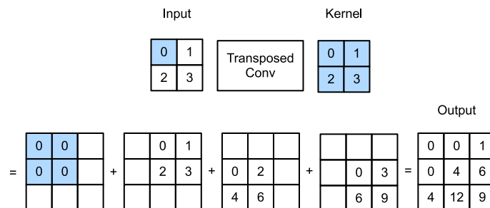
Figure 14.10.1 Transposed convolution with a 2 \times 2 kernel. The shaded portions are a portion of an intermediate tensor as well as the input and kernel tensor elements used for the computation.
