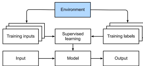
Figure 1.3.6 Collecting data for supervised learning from an environment.
