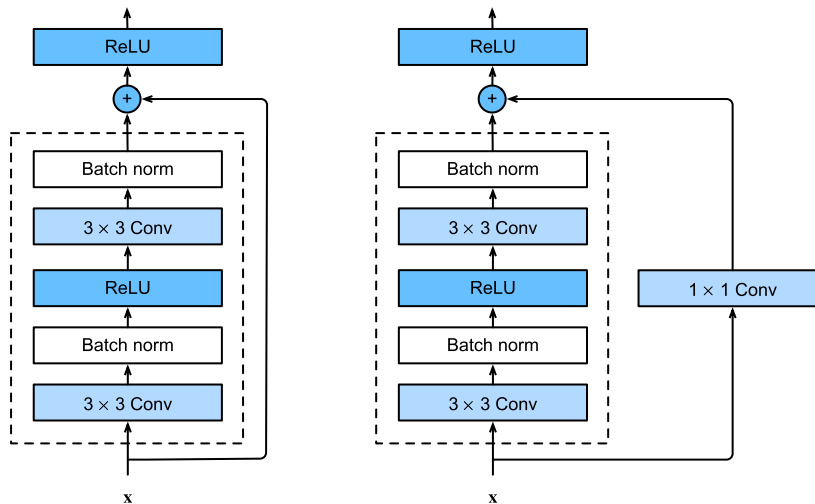
Figure 8.6.3 ResNet block with and without 1 \times 1 convolution, which transforms the input into the desired shape for the addition operation.
