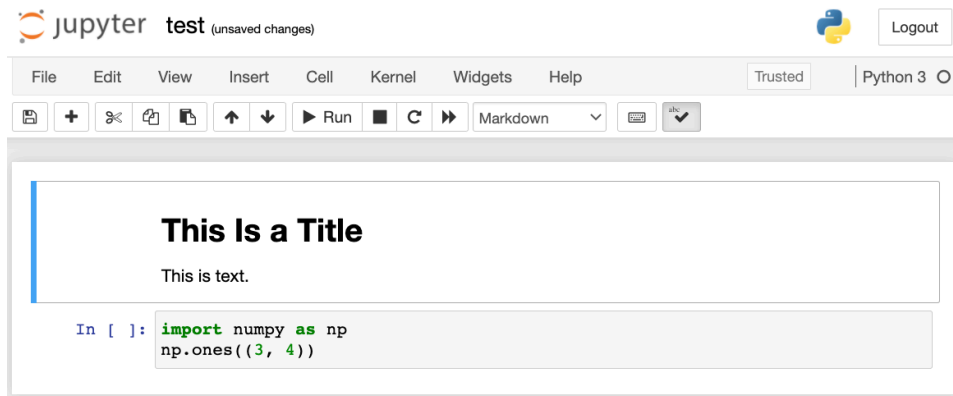
Figure 20.1.2 Markdown and code cells in the text.ipynb file.
