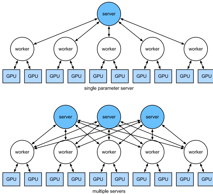
Figure 13.7.8 Top: a single parameter server is a bottleneck since its bandwidth is finite. Bottom: multiple parameter servers store parts of the parameters with aggregate bandwidth.
