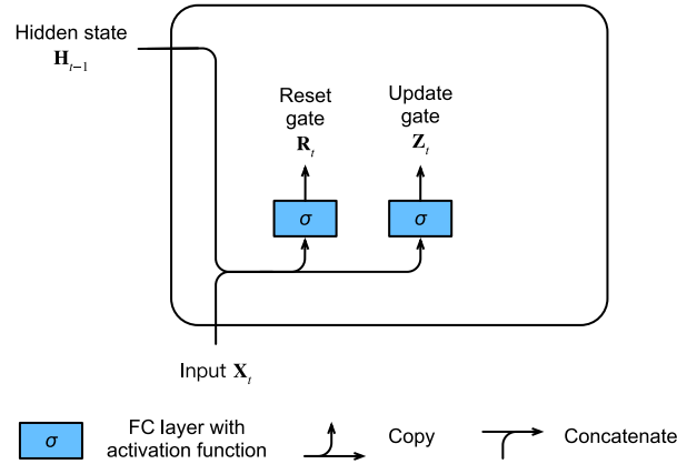
Figure 10.2.1 Computing the reset gate and the update gate in a GRU model.
