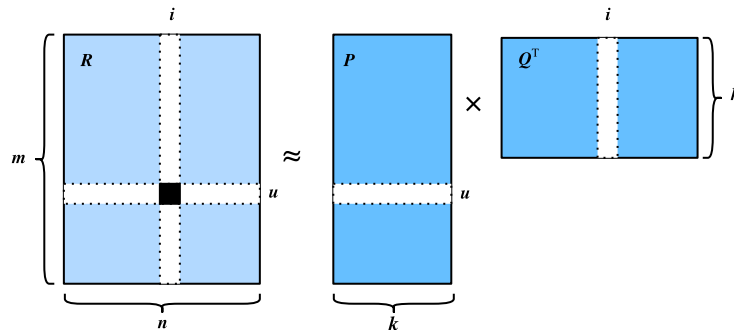
Figure 17.3.1 Illustration of matrix factorization model
