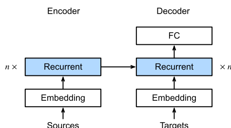
Figure 10.7.2 Layers in an RNN encoder-decoder model.
