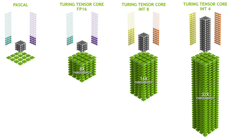
Figure 13.4.9 NVIDIA tensor cores in Turing (image courtesy of NVIDIA).
