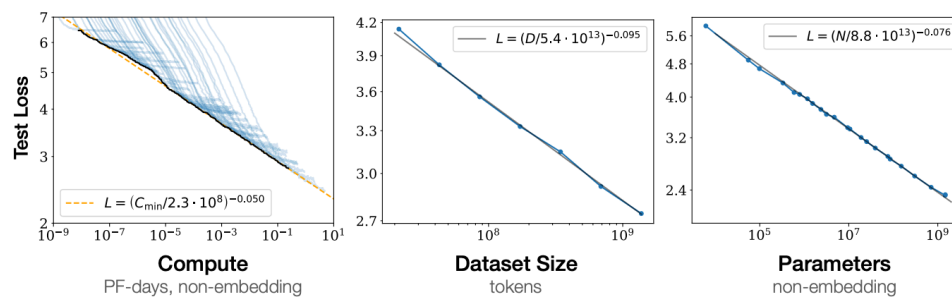
Figure 11.8.9 Transformer language model performance improves smoothly as we increase the model size, dataset size, and amount of compute used for training. For optimal performance all three factors must be scaled up in tandem. Empirical performance has a power-law relationship with each individual factor when not bottlenecked by the other two (caption adapted and figure taken from Kaplan et al. (2020)).
