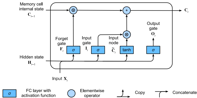
Figure 10.1.3 Computing the memory cell internal state in an LSTM model.
