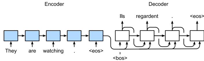
Figure 10.7.3 Predicting the output sequence token by token using an RNN encoder-decoder.
