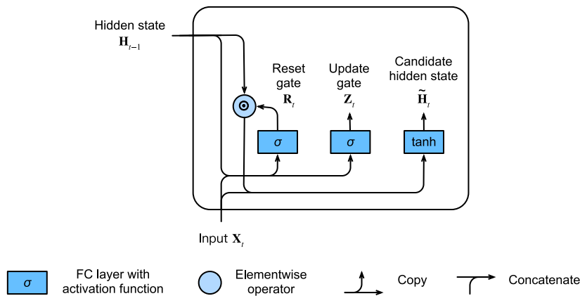
Figure 10.2.2 Computing the candidate hidden state in a GRU model.
