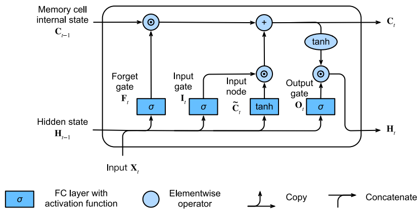
Figure 10.1.4 Computing the hidden state in an LSTM model.
