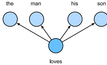
Figure 15.1.1 The skip-gram model considers the conditional probability of generating the surrounding context words given a center word.
