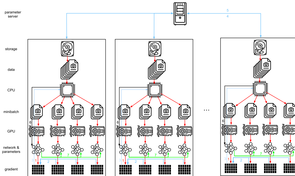
Figure 13.7.7 Multi-machine multi-GPU distributed parallel training.
