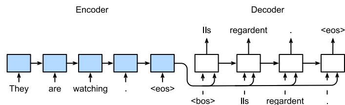
Figure 10.7.1 Sequence to sequence learning with an RNN encoder and an RNN decoder.
