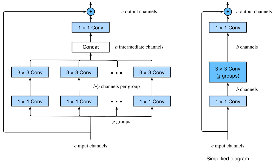
Figure 8.6.5 The ResNeXt block. The use of grouped convolution with g groups is g times faster than a dense convolution. It is a bottleneck residual block when the number of intermediate channels b is less than c .
