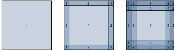
Figure 7.3.1 Pixel utilization for convolutions of size 1 \times 1 , 2 \times 2 , and 3 \times 3 respectively.
