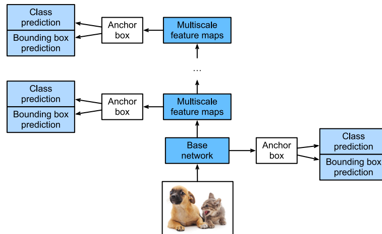
Figure 14.7.1 As a multiscale object detection model, single-shot multibox detection mainly consists of a base network followed by several multiscale feature map blocks.
