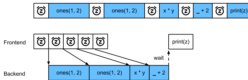
Figure 13.2.3 Interactions of the frontend and backend.
