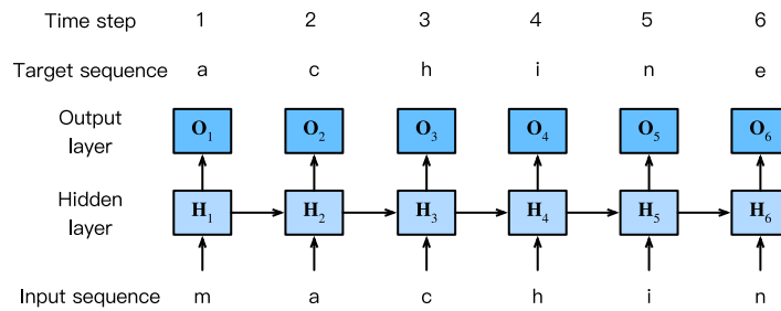
Figure 9.4.2 A character-level language model based on the RNN. The input and target sequences are machin and achine, respectively.
