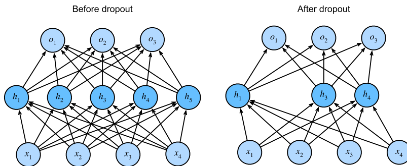
Figure 5.6.1 MLP before and after dropout.
