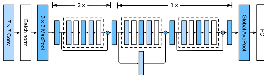
Figure 8.6.4 The ResNet-18 architecture.
