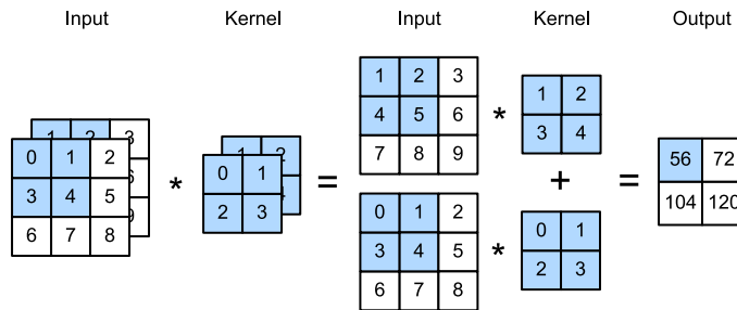
Figure 7.4.1 Cross-correlation computation with 2 input channels.
