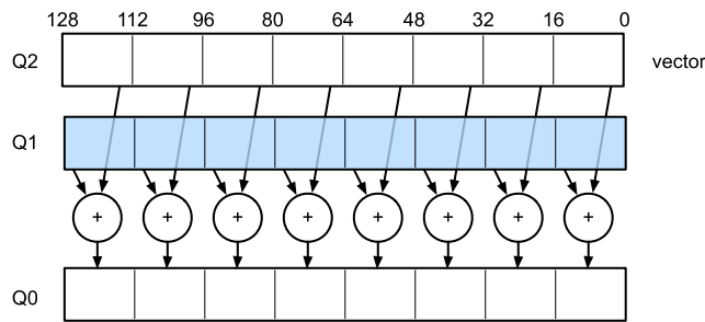
Figure 13.4.5 128 bit NEON vectorization.
