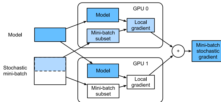
Figure 13.5.3 Calculation of minibatch stochastic gradient descent using data parallelism on two GPUs.
