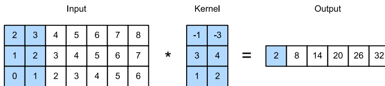
Figure 16.3.4 Two-dimensional cross-correlation operation with a single input channel. The shaded portions are the first output element as well as the input and kernel tensor elements used for the output computation: 2 \times (-1) + 3 \times (-3) + 1 \times 3 + 2 \times 4 + 0 \times 1 + 1 \times 2 = 2 .
