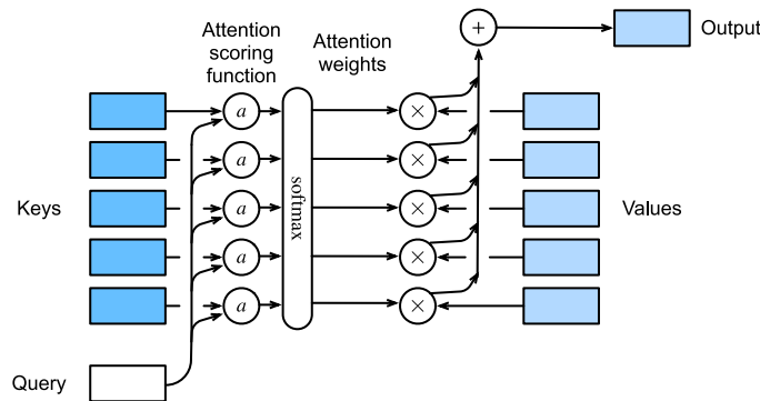
Figure 11.3.1 Computing the output of attention pooling as a weighted average of values.
