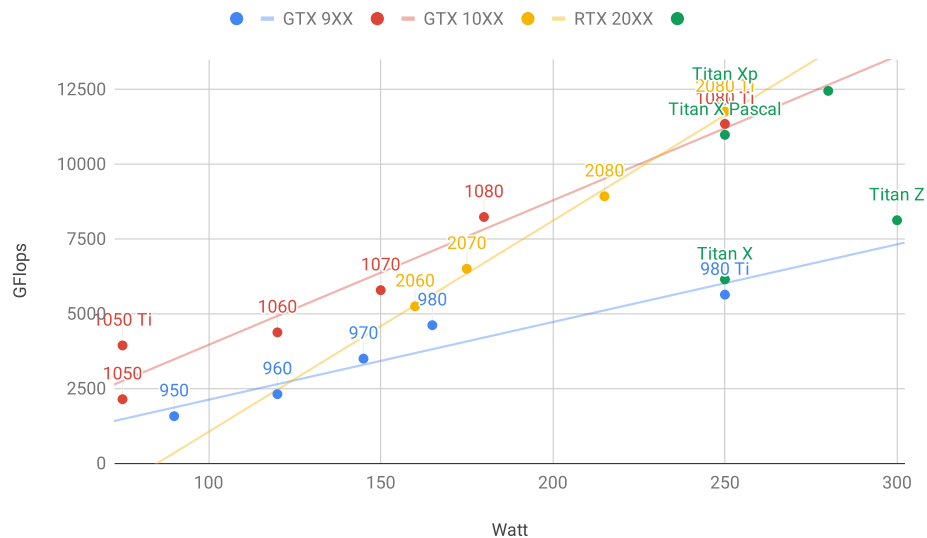
Figure 20.5.2 Floating-point compute power and energy consumption.
