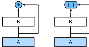
Figure 8.7.1 The main difference between ResNet (left) and DenseNet (right) in cross-layer connections: use of addition and use of concatenation.
