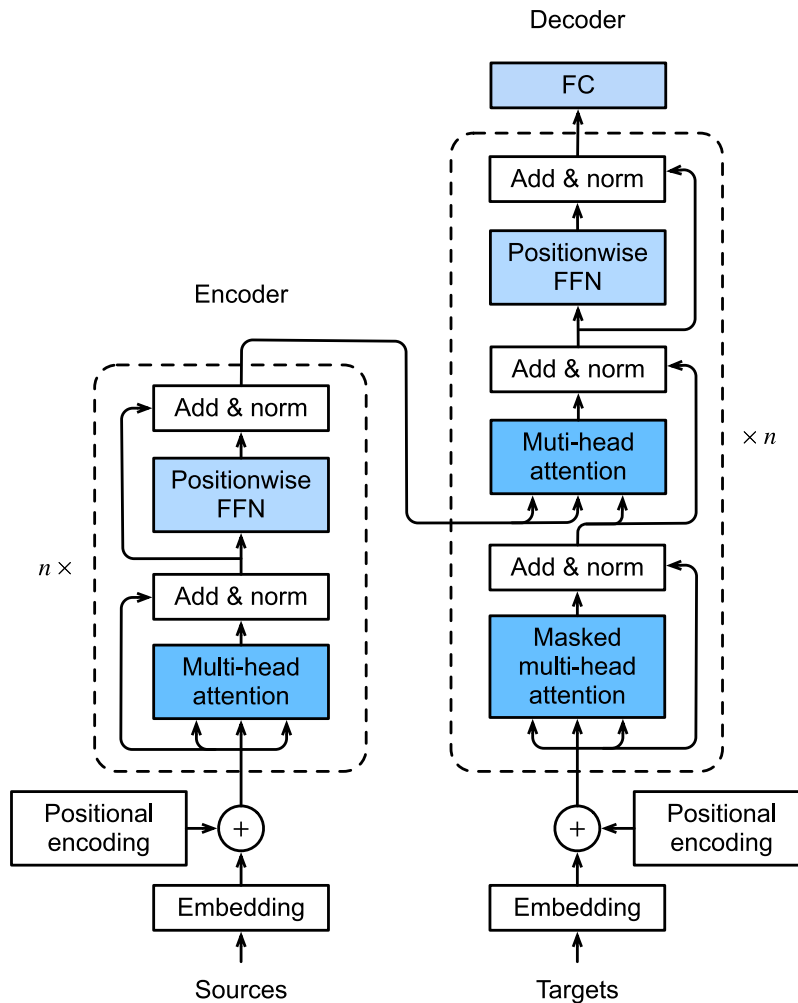
Figure 11.7.1 The transformer architecture.
