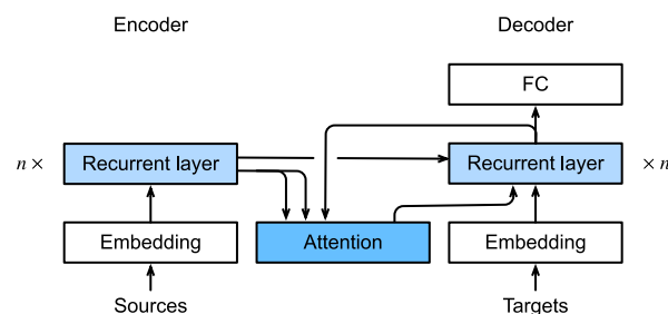
Figure 11.4.1 Layers in an RNN encoder-decoder model with Bahdanau attention.
