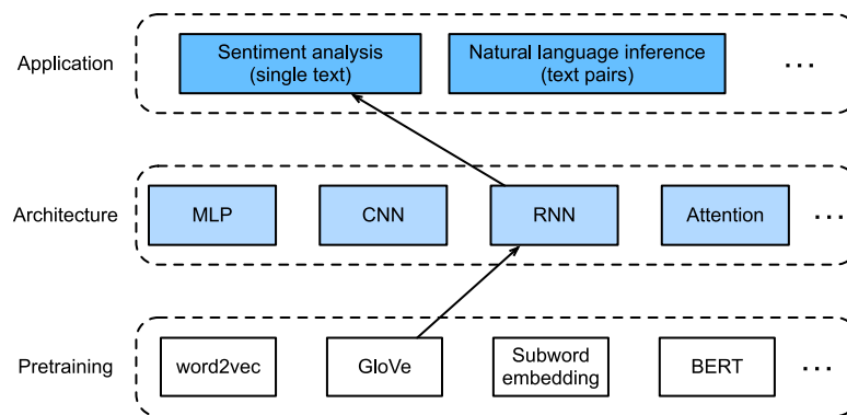
Figure 16.2.1 This section feeds pretrained GloVe to an RNN-based architecture for sentiment analysis.
