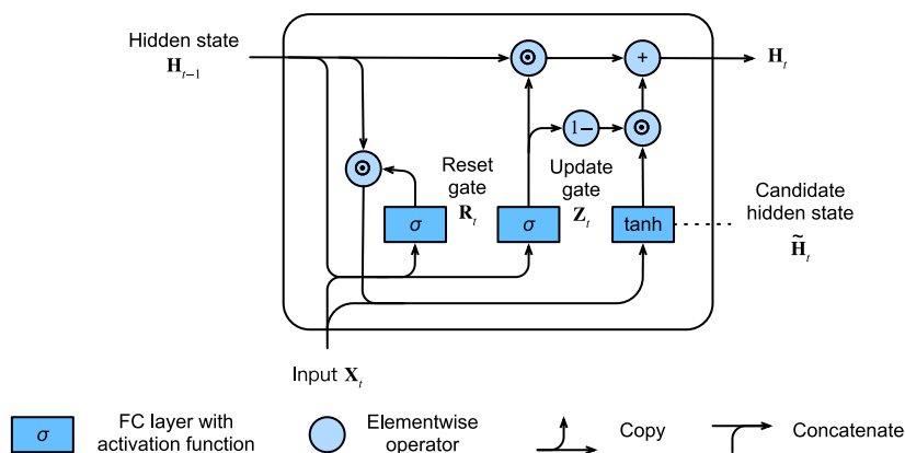
Figure 10.2.3 Computing the hidden state in a GRU model.
