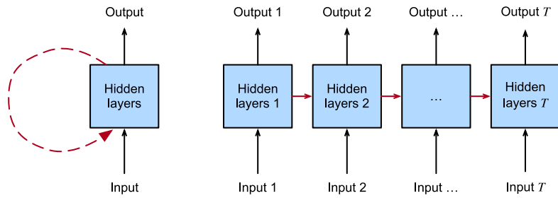
Figure 9.1 On the left recurrent connections are depicted via cyclic edges. On the right, we unfold the RNN over time steps. Here, recurrent edges span adjacent time steps, while conventional connections are computed synchronously.
