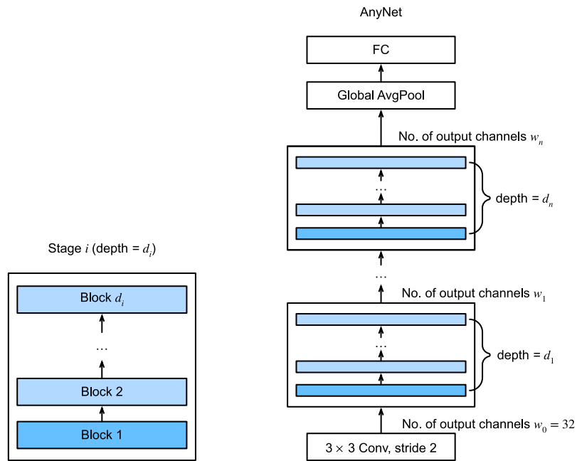
Figure 8.8.1 The AnyNet design space. Besides the number of groups and bottleneck ratio within each block, design choices include depth d_i and the number of output channels w_i for any stage i .
