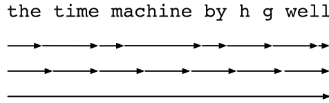
Figure 9.7.1 Comparing strategies for computing gradients in RNNs. From top to bottom: randomized truncation, regular truncation, and full computation.
