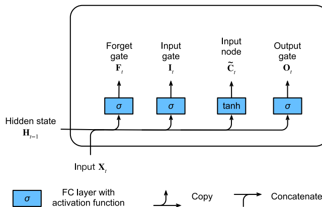
Figure 10.1.2 Computing the input node in an LSTM model.
