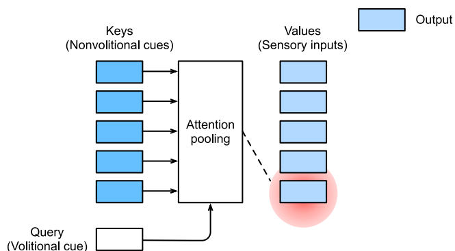
Figure 11.1.3 Attention mechanisms bias selection over values (sensory inputs) via attention pooling, which incorporates queries (volitional cues) and keys (nonvolitional cues).
