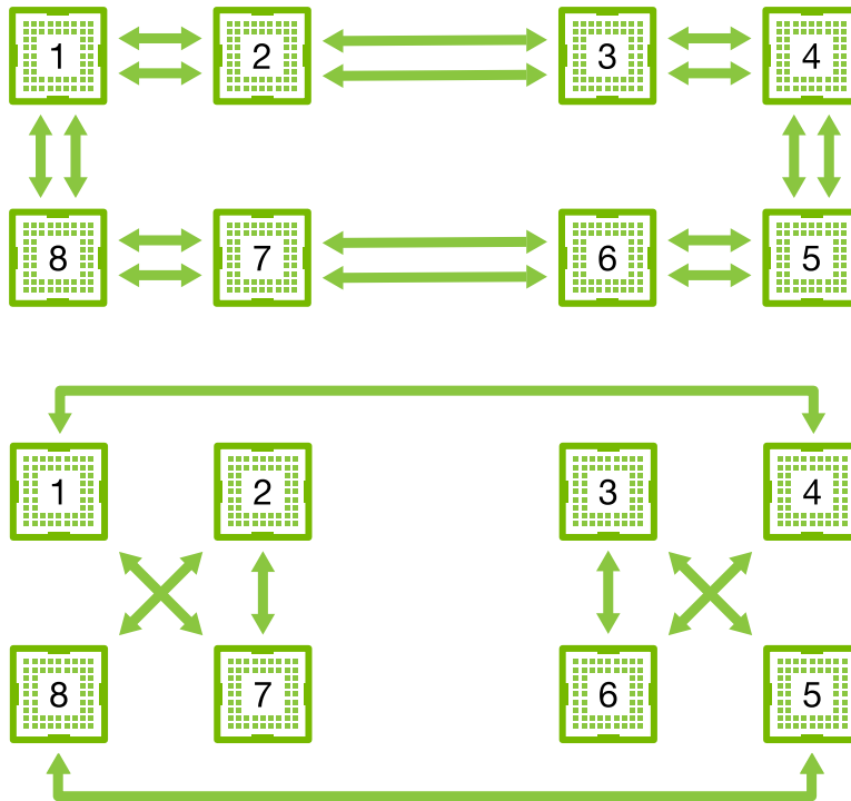
Figure 13.7.5 Decomposition of the NVLink network into two rings.
