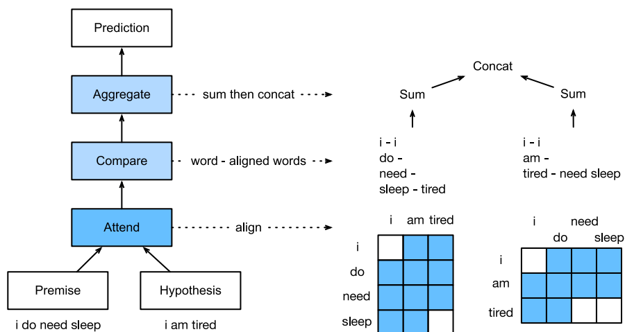
Figure 16.5.2 Natural language inference using attention mechanisms.
