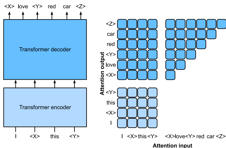
Figure 11.8.3 Left: Pretraining T5 by predicting consecutive spans. The original sentence is I, love, this, red, car, where love is replaced by a special <X> token, and consecutive red, car are replaced by a special <Y> token. The target sequence ends with a special <Z> token. Right: Attention pattern in the transformer encoder-decoder. In the encoder self-attention (lower square), all input tokens attend to each other; In the encoder-decoder cross-attention (upper rectangle), each target token attends to all input tokens; In the decoder self-attention (upper triangle), each target token attends to present and past target tokens only (causal).
