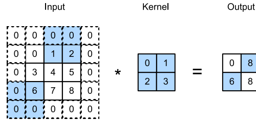
Figure 7.3.3 Cross-correlation with strides of 3 and 2 for height and width, respectively.
