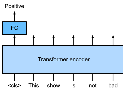
Figure 11.8.2 Fine-tuning BERT for sentiment analysis.
