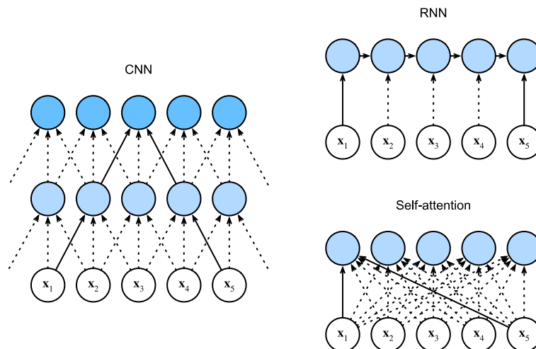
Figure 11.6.1 Comparing CNN (padding tokens are omitted), RNN, and self-attention architectures.
