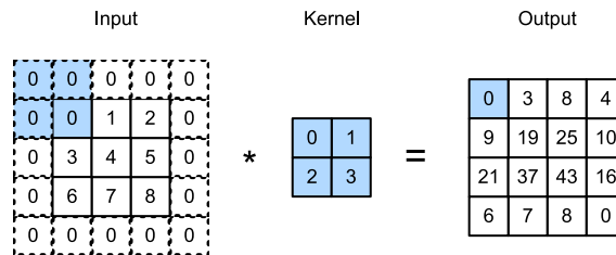
Figure 7.3.2 Two-dimensional cross-correlation with padding.
