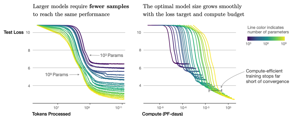
Figure 11.8.10 Transformer language model training runs (figure taken from Kaplan et al. (2020)).
