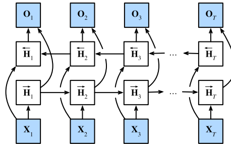
Figure 10.4.1 Architecture of a bidirectional RNN.
