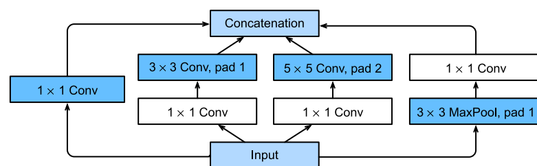
Figure 8.4.1 Structure of the Inception block.
