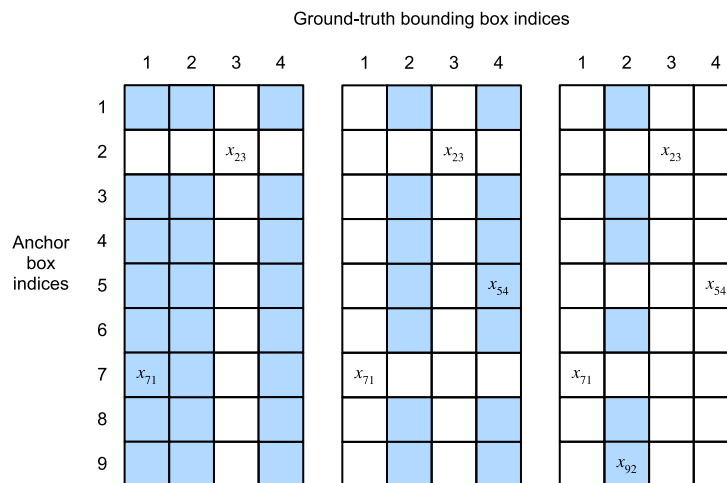
Figure 14.4.2 Assigning ground-truth bounding boxes to anchor boxes.
