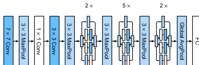
Figure 8.4.2 The GoogLeNet architecture.
