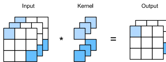
Figure 7.4.2 The cross-correlation computation uses the 1 \times 1 convolution kernel with 3 input channels and 2 output channels. The input and output have the same height and width.
