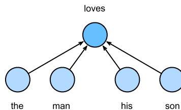
Figure 15.1.2 The continuous bag of words model considers the conditional probability of generating the center word given its surrounding context words.
