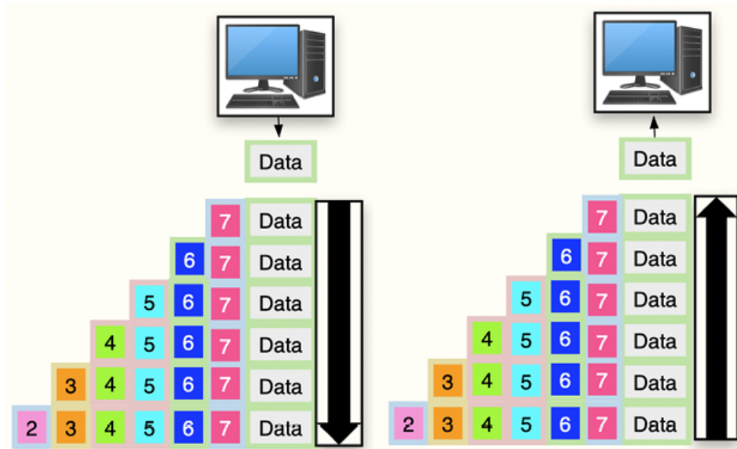
Figure 11.3: Encapsulation
