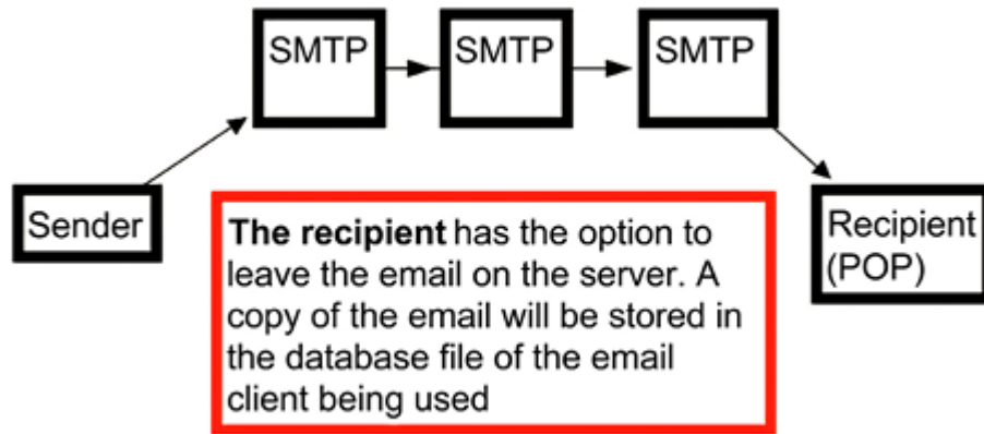
Figure 8.2: SMTP-POP map
