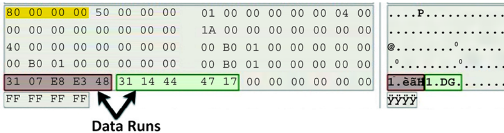
Figure 4.45: Run list
