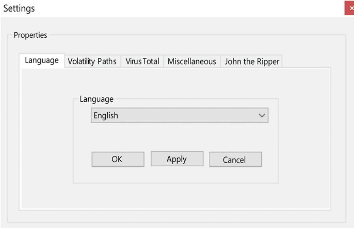
Figure 7.14: Volix settings
