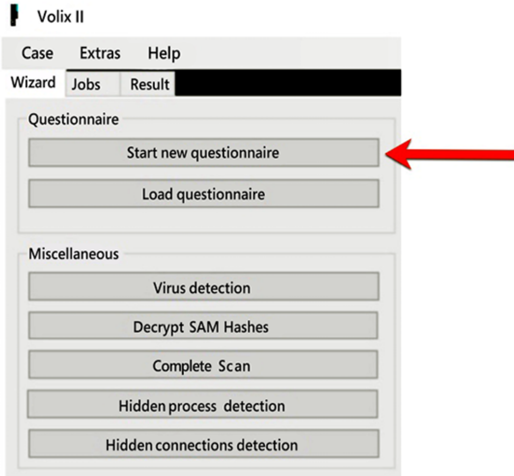
Figure 7.16: VOLIX wizard
