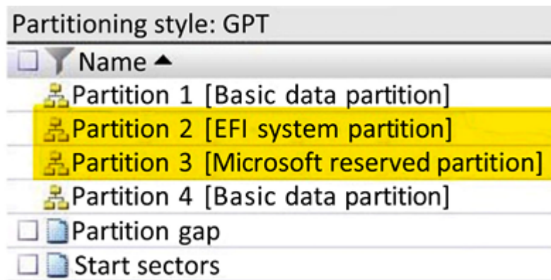
Figure 4.14: HPA 1
