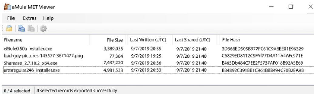
Figure 9.33: MetViewer
