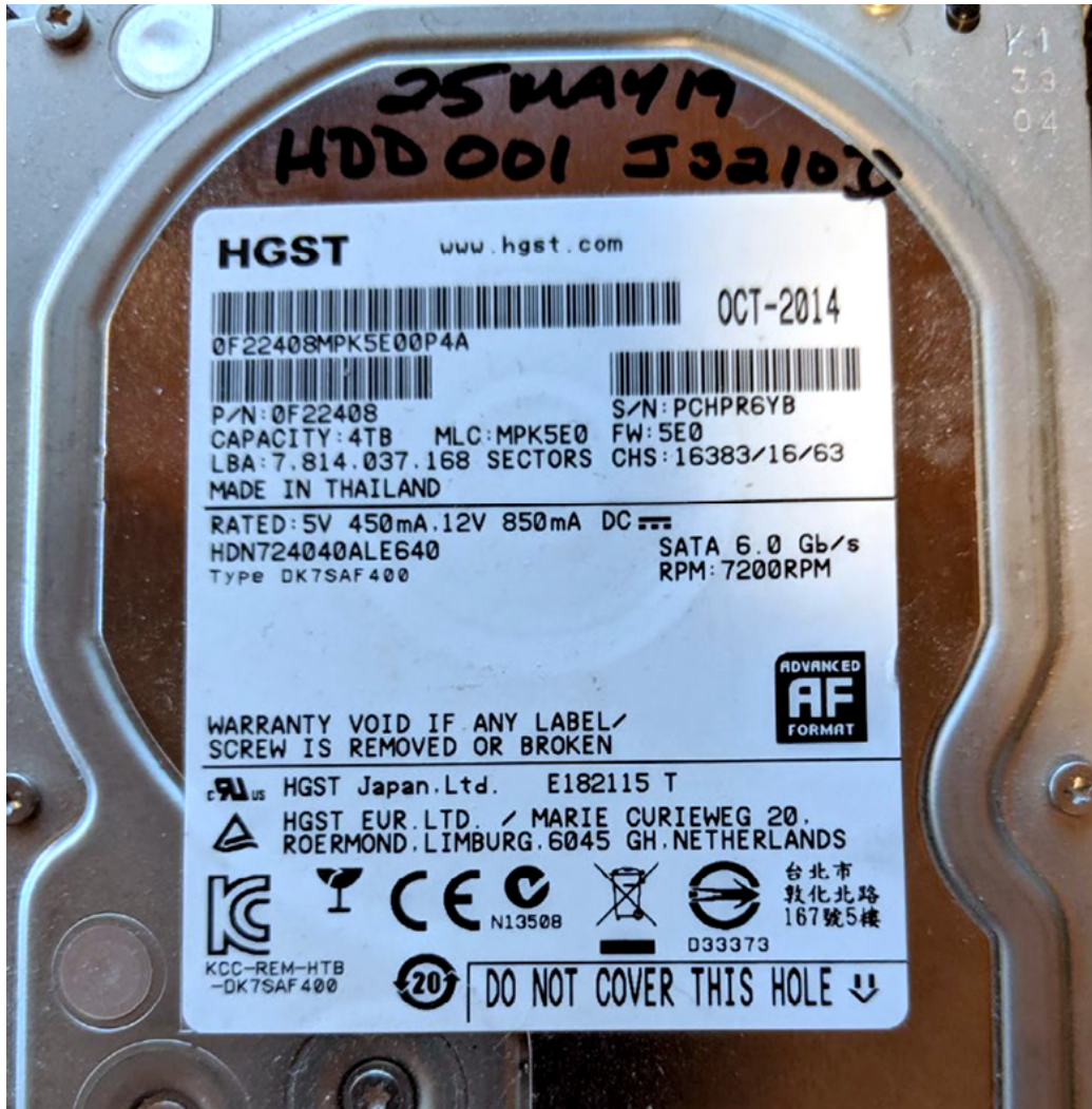
Figure 2.3: A hard drive
