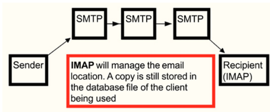
Figure 8.3: IMAP map
