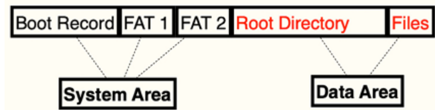
Figure 4.16: FAT areas
