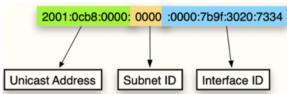
Figure 11.9: IPv6
