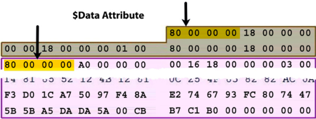
Figure 4.39: $Data Attribute
