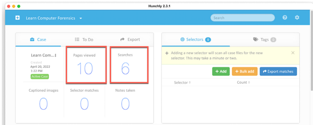
Figure 10.22: Hunchly desktop
