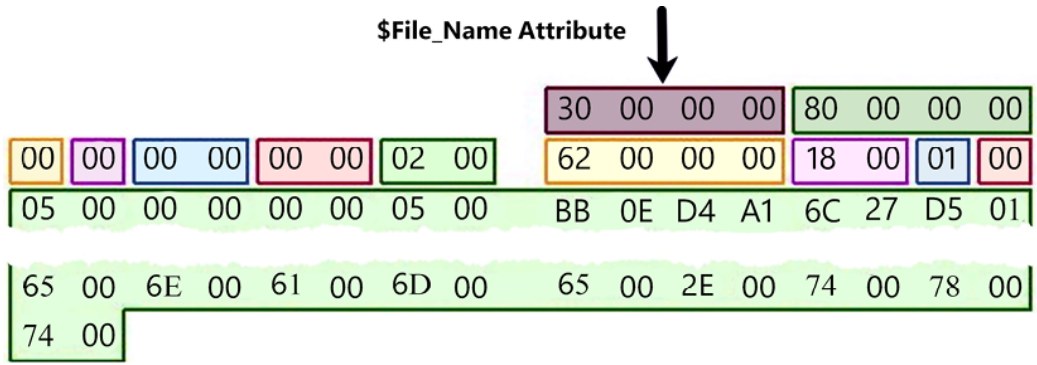
Figure 4.37: $File_Name Attribute
