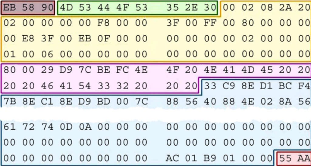
Figure 4.17: VBR
