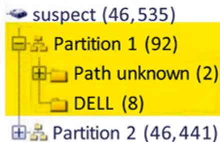
Figure 4.15: HPA 2
