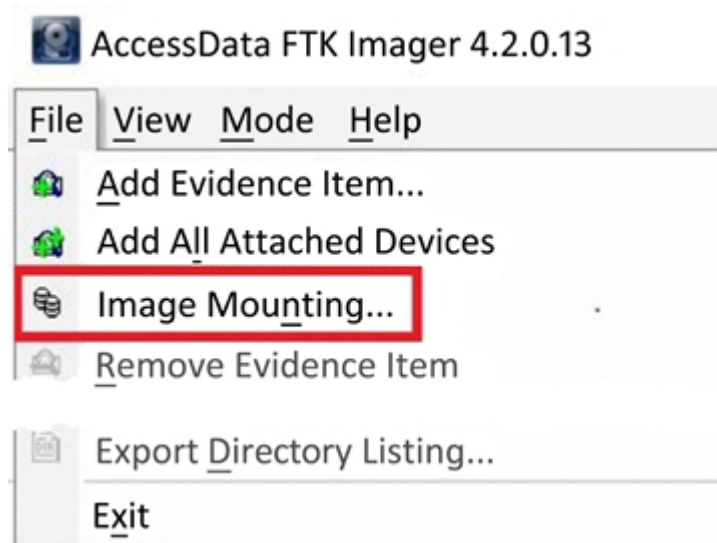
Figure 2.12: Image mounting
