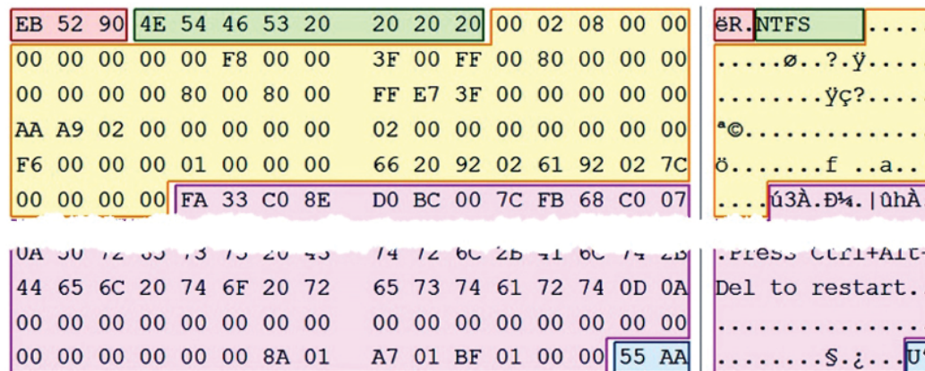
Figure 4.30: NTFS VBR
