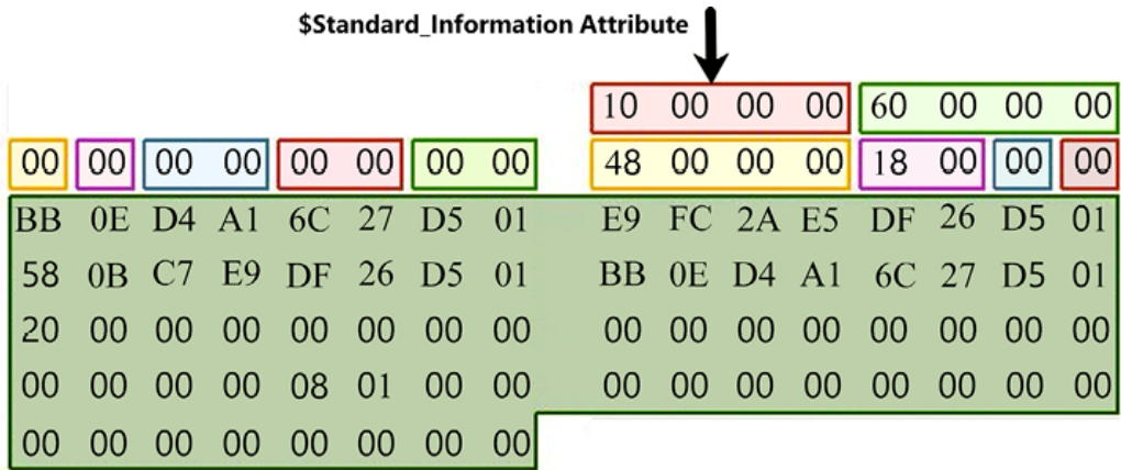
Figure 4.35: $Standard_Information Attribute
