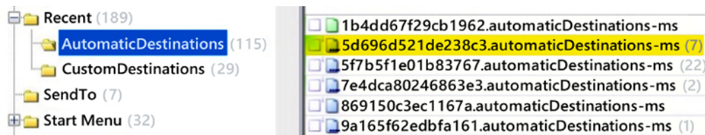
Figure 6.24: JumpList display
