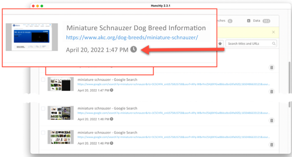
Figure 10.23: Hunchly history
