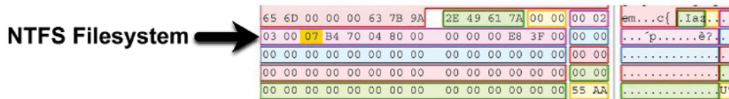
Figure 4.29: NTFS MBR
