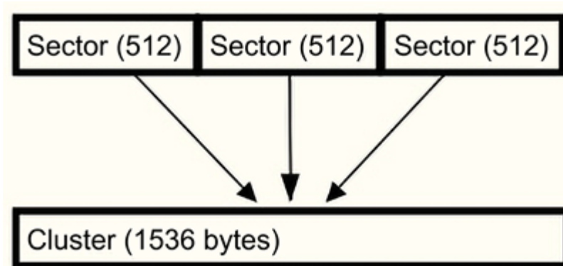
Figure 4.18: Cluster example
