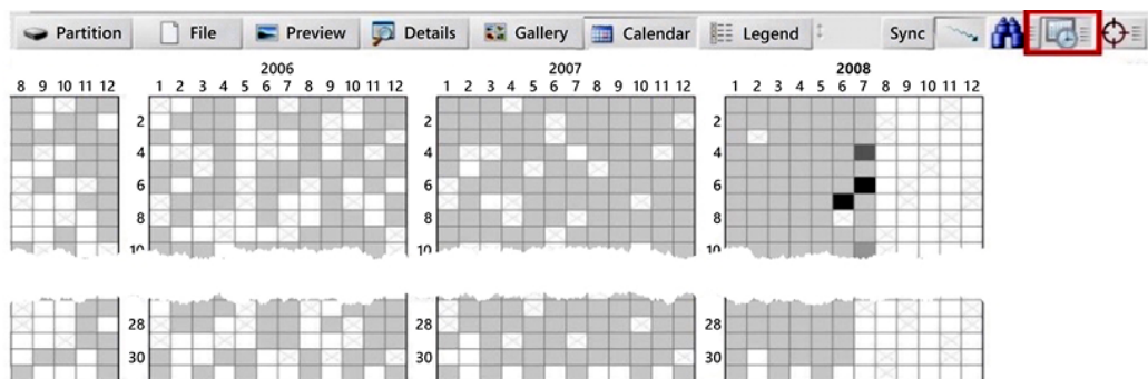
Figure 5.1: X-Ways
