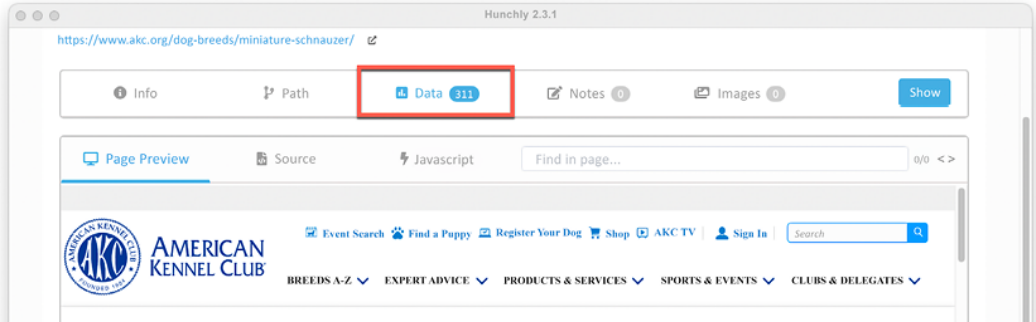
Figure 10.24: Hunchly preview
