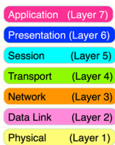
Figure 11.1: OSI model
