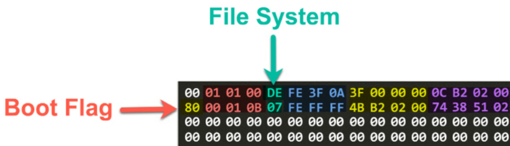
Figure 4.6: Partition tables
