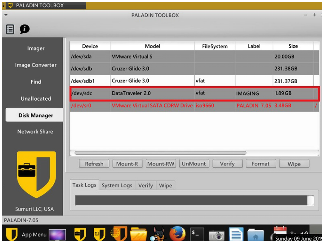
Figure 3.32: PALADIN toolbox
