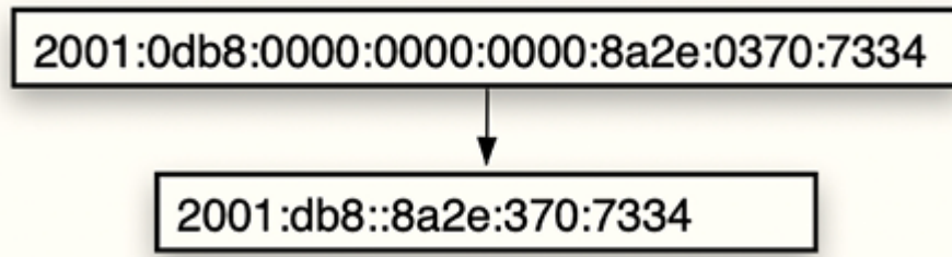
Figure 11.10: IPv6 shorthand example
