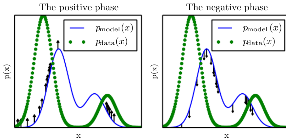
Figure 18.1: The view of algorithm 18.1 as having a “positive phase” and “negative phase.” ( Left ) In the positive phase, we sample points from the data distribution, and push up on their unnormalized probability. This means points that are likely in the data get pushed up on more. ( Right ) In the negative phase, we sample points from the model distribution, and push down on their unnormalized probability. This counteracts the positive phase’s tendency to just add a large constant to the unnormalized probability everywhere. When the data distribution and the model distribution are equal, the positive phase has the same chance to push up at a point as the negative phase has to push down. When this occurs, there is no longer any gradient (in expectation) and training must terminate.
