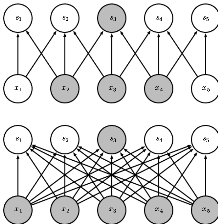
Figure 9.3: Sparse connectivity, viewed from above: We highlight one output unit, s_3 , and also highlight the input units in \mathbf{x} that affect this unit. These units are known as the receptive field of s_3 . (Top)When \mathbf{s} is formed by convolution with a kernel of width 3, only three inputs affect s_3 . (Bottom)When \mathbf{s} is formed by matrix multiplication, connectivity is no longer sparse, so all of the inputs affect s_3 .
