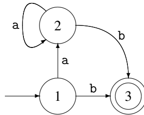
Figure 2.8: Example of a DFA
