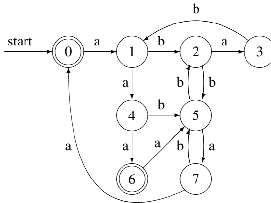
Figure 2.10: Non-minimal DFA
